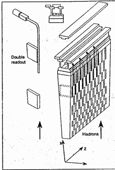
Figure 1: Principle of the tile hadronic calorimeter.
