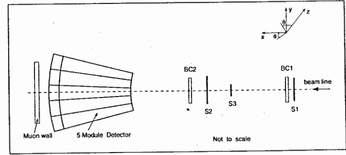
Figure 2: Setup of the tile hadronic calorimeter prototype.
