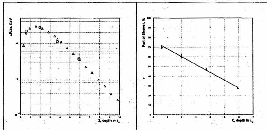
Figure 11: Left: Longitudinal profile as a function of longitudinal coordinate x in units \lambda_{\pi}^{Fe} . Open circle – our data, open triangle – data for conventional calorimeter, diamond – Monte Carlo prediction. Right: The fractions of the “electromagnetic” parts of showers in various depths as a function of x .
