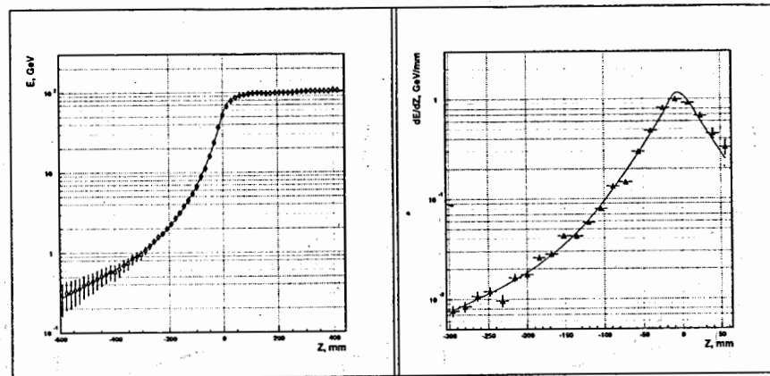
Figure 7: Left: The cumulative function f(z) for overall calorimeter. Curves are fits of equations (16) and (17) to the data. Right: The marginal density f'(z) for overall calorimeter.
