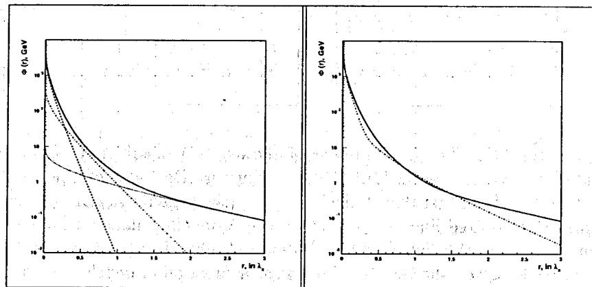
Figure 9: Left: The radial energy density as a function of r (in units of \lambda_f ) for TILECAL (solid line), the contribution to \Phi(r) from the first term (dashed line), the contribution to \Phi(r) from the second term (dash-dotted line), the contribution to \Phi(r) from the third term (dotted line). Right: The comparison of the radial energy densities as a function of r (in units of \lambda_f ) for TILECAL (solid line) and SPACAL (dash-dotted line).
