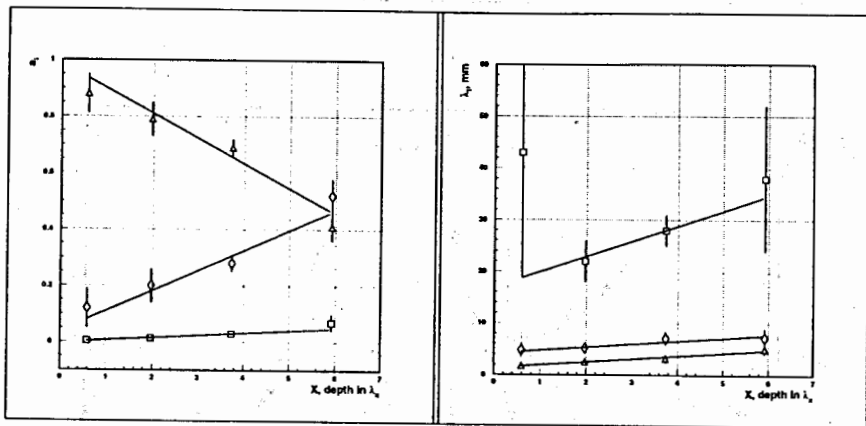
Figure 5: The shower depth dependences of the parameters a_i and \lambda_i .
