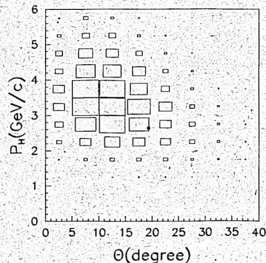
Figure 5: The expected angular and momentum distributions of H dihyperons produced within a fireball ( T_B=150 MeV) in central MgMg-collisions ( the black circle—the detected event ).
