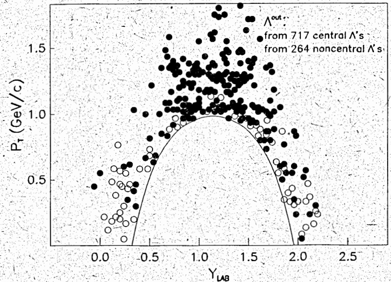
Figure 2: P_T - Y_L -plot for cumulative \Lambda hyperons produced: in non central HeLi CC-collisions selected from 264 \Lambda 's (open circles) and in central CNe, ONe, CCu, CZr, MgMg collisions from 717 \Lambda 's (black circles) at momenta 4.2 - 4.5 A GeV/c outside kinematical limits for NN interactions, outlined by solid lines
