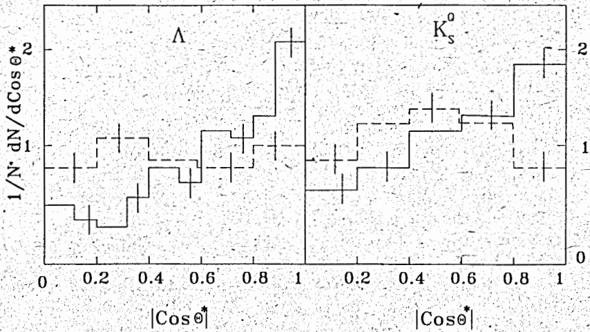
Figure 1: Folded (in \text{Cos } \theta^* ) angular distributions of \Lambda hyperons and K_S^0 -mesons produced: in noncentral CC-collisions — solid lines, and in central ones — dashed lines.
