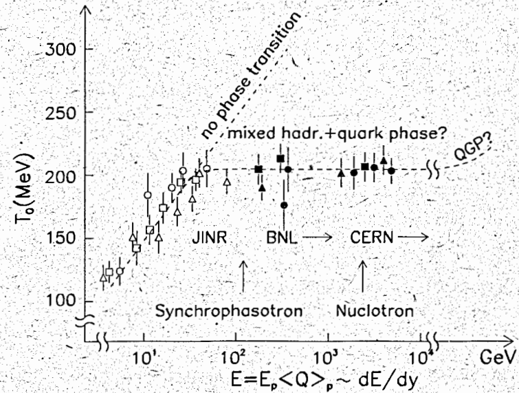
Figure 4: Inverse slope parameters T_0 versus E = E_p \langle Q \rangle : open circles, open triangles and open squares - K_S^0 , \Lambda and proton JINR data; black circles, black triangles and black squares - neutral (charged) kaons, \Lambda and proton data of BNL (17) and CERN (18). To make an adequate comparison, the T_0 parameters (not the Boltzmann temperatures T_B ) are shown on this figure, because T_B values are not given in CERN papers.
