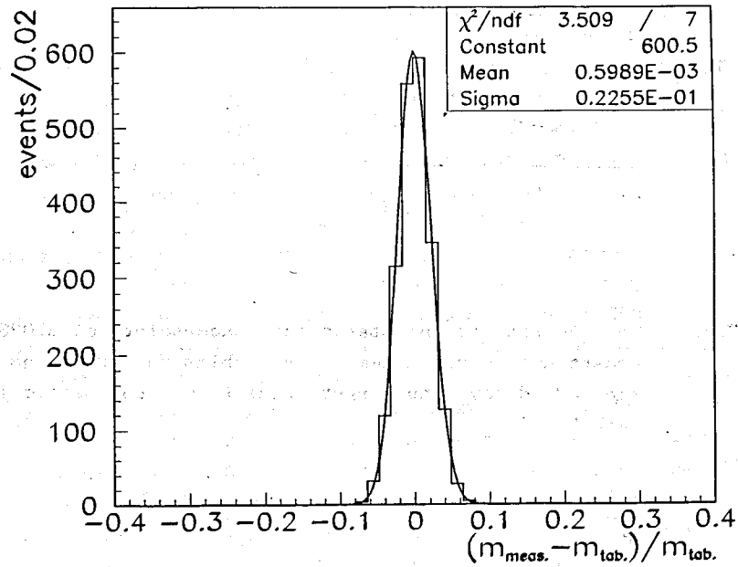
Fig.3 Distribution of quantity (m_{meas.} - m_{tab.})/m_{tab.} (see the text). Also, the fitting result is shown.
