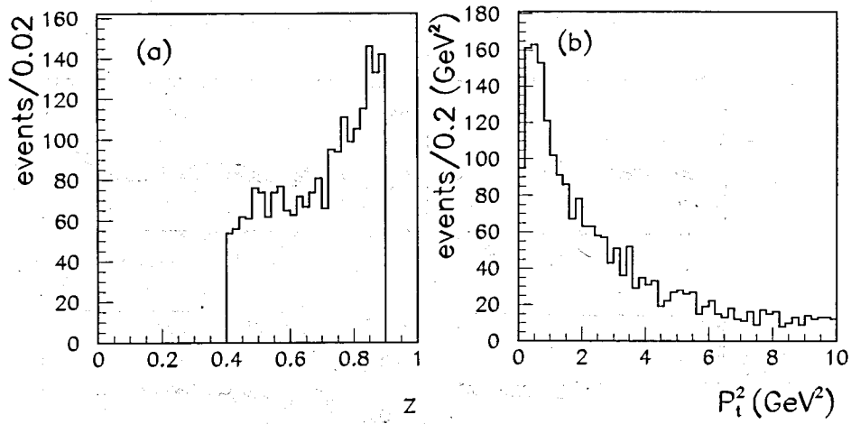
Fig.2 Z (a)- and P_T^2 (b) - distributions for J/\psi produced in \mu N \rightarrow \mu^* J/\psi X via photon-gluon fusion mechanism.
