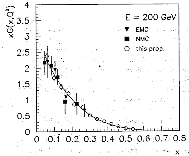
Fig.4 The normalized gluon distribution, xG(x, Q^2) (only statistical errors are shown) together with the J/\psi data from EMC[9] and NMC[10]. The curve presents the fitted parametrization of the simulated data.
