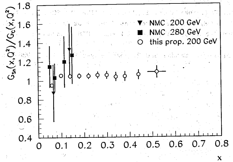
Fig.5 The ratio of gluon distributions on tin and carbon from simulated data(see the text).
