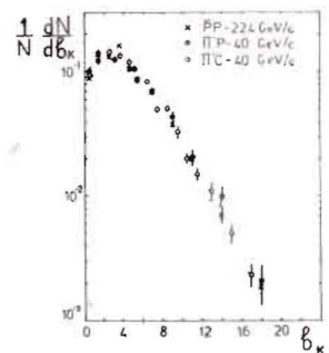
Fig.1. The b_k distribution of \pi^- mesons in jets for the fragmentation of different projectiles ( x_p \geq 0.1, x_t \leq 0.1 ) and targets ( x_t \geq 0.1, x_p \leq 0.1 ).
