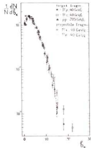
Fig.1. The b_k distribution of \pi^- mesons in jets for the fragmentation of different projectiles ( x_p \geq 0.1, x_t \leq 0.1 ) and targets ( x_t \geq 0.1, x_p \leq 0.1 ).
