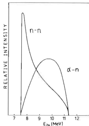
Fig. 2. Event distribution for the reaction tt\mu \rightarrow {}^4\text{He}+2n+\mu over the total energy of two neutrons.
