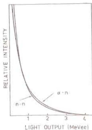
Fig. 1. Amplitude distributions of neutrons for reaction (2), calculated for the detector with 1 l of the NE-213 scintillator.
