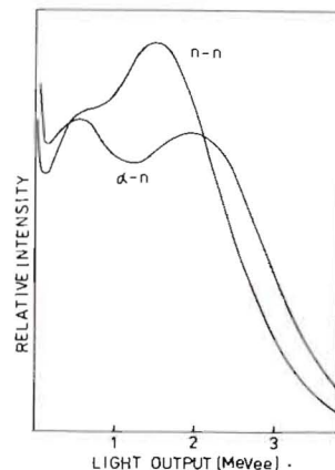
Fig. 3. Amplitude distributions of neutrons for reaction (2), calculated for the detector with 200 l of the NE-213 scintillator.
