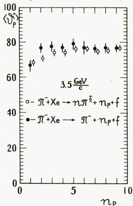
Fig. 3. Proton emission average angle \langle \theta_p \rangle in dependence on the multiplicity n_p of fast protons, of kinetic energy from about 20 to about 400 MeV, emitted in two samples of pion-xenon nucleus collision events at 3.5 GeV/c momentum: full circles - in the sample of collisions without particle production, when incident pion is absorbed inside the target nucleus or deflected in passage through it; empty circles - in the sample of any-type collisions, n - number of secondary pions, f - residual nuclear fragments.
