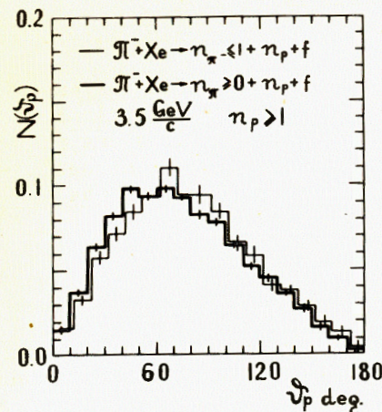
Fig.1. Distributions N(\theta_p) of the emission angles \theta_p of fast protons, of kinetic energy from about 20 to about 400 MeV, emitted in pion-xenon nucleus collisions at 3.5 GeV/c momentum: — - in the sample of events without particle production, when incident pion is absorbed inside the target nucleus or deflected in traversing it; — in the sample containing any-type collision events, with particle production and without particle production. n_\pi - multiplicity of secondary pions, n_p - multiplicity of emitted protons, f - residual nuclear fragments.
