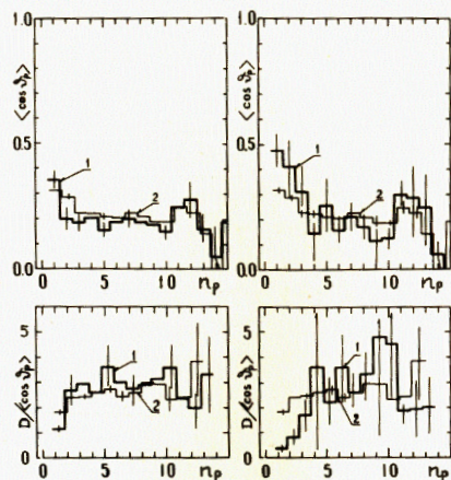
Fig. 4. Average cosine \langle \cos \theta_p \rangle and corresponding normalized dispersion D/\langle \cos \theta_p \rangle in dependence on multiplicity n_p of fast protons, of kinetic energy from about 20 to about 400 MeV, emitted in pion-xenon nucleus collisions at 3.5 GeV/c momentum through emission angles \theta_p : left side - in the sample of any-type collision events, histogram 2, and in the sample of collision events without particle production when incident pion is absorbed inside the target nucleus or deflected in passage through it, histogram 1, right side - in the sample of any-type collision events, histogram 2, and in the sample of collision events without particle production when incident pion is absorbed inside the target nucleus, histogram 1.
