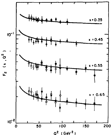
Fig. 2. F_2(x, Q^2) measured with 120 GeV \mu^+ (open symbols) and with 200 GeV \mu^+/\mu^- (closed symbols) using R = 0 . The curves represent the best fit to the data with the Gonzalez-Arroyo et al. parametrization with \Lambda = 85 MeV, \alpha = 0.68 and \beta = 3.65 .
