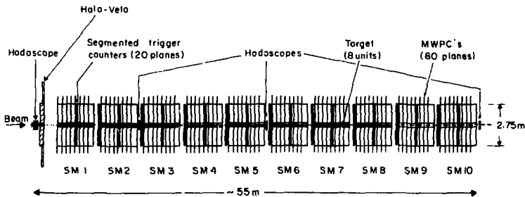
Fig. 1 Schematic view of the experimental set-up. Magnetized iron toroids with interspersed trigger counters and multiple wire proportional chambers are arranged in ten supermodules (SM1-10). The last two supermodules do not contain target units. A wall of scintillation counters vetoes the halo muons.
