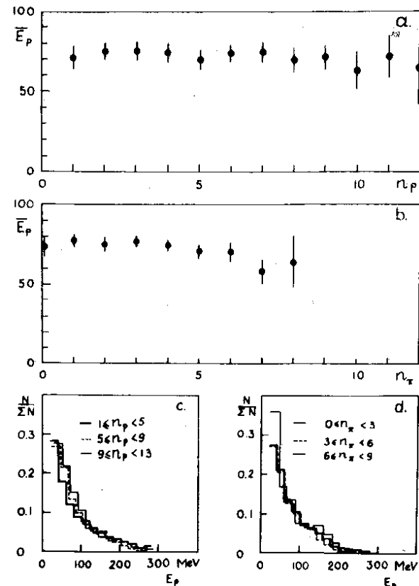
Fig. 2. Energy characteristics of the protons emitted in the pion-xenon nuclei collisions at 3.5 GeV/c; a) average energy of the protons in dependence on the proton multiplicity n_p /1/ ; b) average energy of the protons in dependence on the numbers n_\pi of pions generated /1/ ; c) energy spectra of protons in the classes of pion-xenon nuclei collision events with different numbers n_p of the protons emitted /1/ ; d) energy spectra of protons in the classes of events with different numbers n_\pi of pions generated /1/ .
