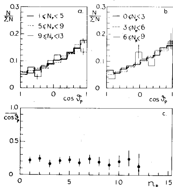
Fig. 3. Angular characteristics of the protons emitted in the pion-xenon nuclei collisions at 3.5 \text{ GeV}/c 1/ : a) distributions of the emission angles \theta_p of protons in the classes of collision events with different numbers N_p of protons emitted; b) distributions of the emission angles of protons emitted in the collision events with different numbers N_\pi of the pion generated; c) \cos\theta_p in dependence on the n_p .
