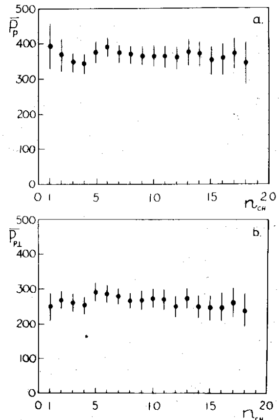
Fig. 4. Average total P_p and transverse P_{p\perp} momenta of the protons emitted in the pion-xenon nuclei collision events at 3.5 \text{ GeV}/c with different numbers n_{ch} of secondaries 4/ .
