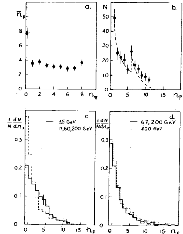
Fig. 1. Proton multiplicity distributions: a) the dependence of the average proton multiplicity \bar{n}_p on the number n_\pi of secondary pions produced in pion-xenon nuclei collisions at 3.5 GeV/c /1/ ; b) the proton multiplicity distribution of the events with zero and one secondary pion without multiparticle production /2/ ; the dotted line presents the calculated distribution /3/ ; c) the proton multiplicity distribution of the pion-xenon /4/ (solid) and the pion-argon-bromine /7/ (dotted) collisions at different energies; d) proton multiplicity distributions in the proton-argon-bromine nuclei collisions at different energies /7/ .
