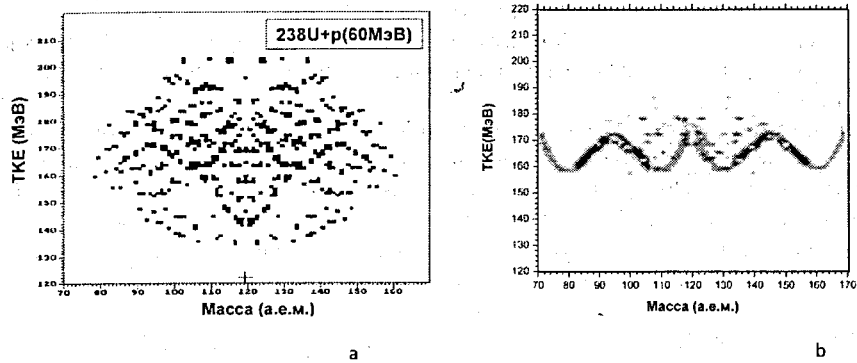
Fig. 4. Fine structure of the M-TKE distribution revealed in the frame of the heuristics approach (a). The same initial data processed using morphological methods of image analysis (b). It is proved the probability of random appearance of the FS to be less than 10^{-3} .
