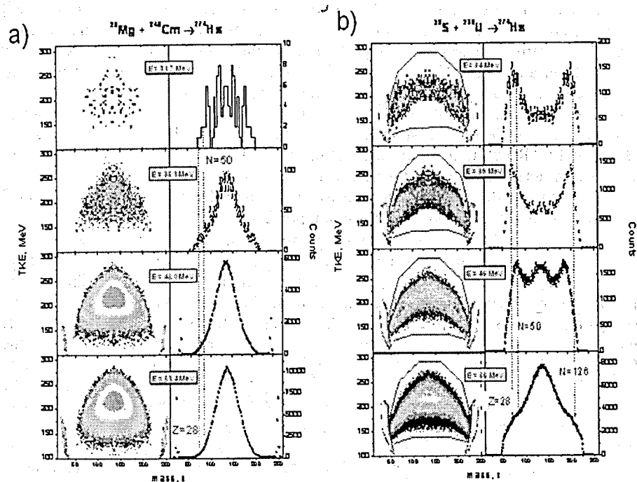
[8]. Fig. 3. The mass-energy distributions of binary products for the reactions ^{26}\text{Mg}+^{248}\text{Cm} (a) and ^{36}\text{S}+^{238}\text{U} (b), leading to the formation of the same compound system ^{274}\text{Hs} at different excitation energies near the Coulomb barrier. The two-dimensional matrices mass-total kinetic energy for binary products are at the left panel; right panel shows the mass distributions of fission-like events inside the outlined contour on the M-TKE matrices.
