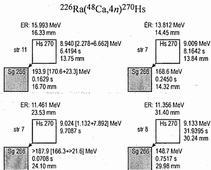
Fig. 1. Decay chains of the nuclei ^{270}\text{Hs} and ^{266}\text{Sg} at the ^{48}\text{Ca} energy of 233 MeV.
