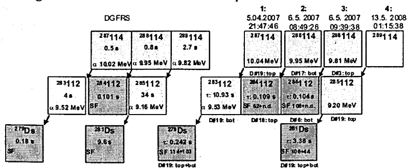
Fig. 2. The decay properties of ^{287-289}\text{114} .
