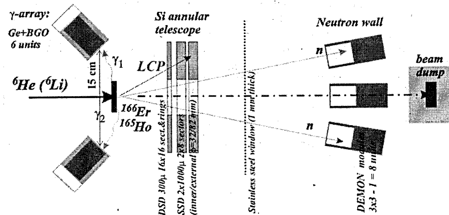
Fig. 5. Scheme of experiments for the complete and incomplete fusion study.
