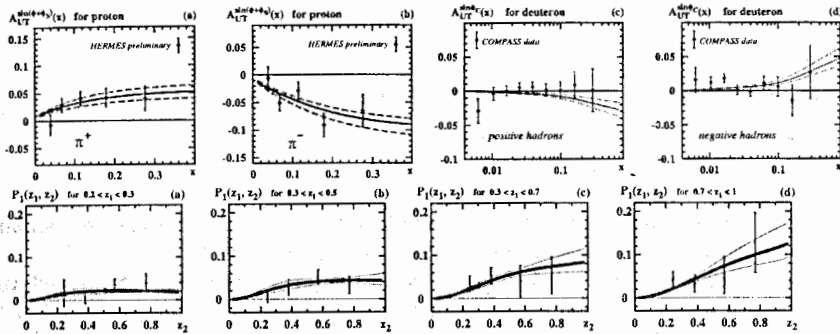
Fig. 1: Top: The HERMES (a,b) and COMPASS (c,d) data on Collins asymmetry. Bottom: The BELLE data on Collins effect.
