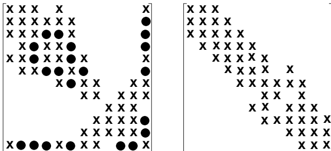
FIGURE 3.6. Factors L and U after the direct (left) and reverse (right) Cuthill-McKee reordering. In the second case, fill-in is absent
