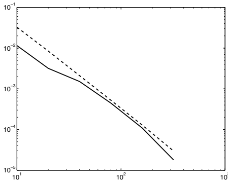
FIGURE 13.3. Convergence analysis for the dG(1)cG(1) method. The solid line is the time discretization error while the dashed line is the space discretization error. In the first case the x -axis denotes the number of time steps while in second case it represents the number of space subintervals
