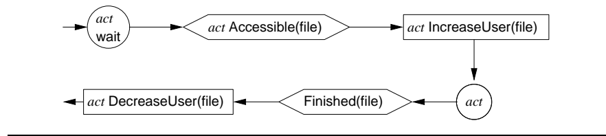
Fig. 6.2 Basic MULTIPLEREADONEWRITE ASM ( act=Read,Write )
