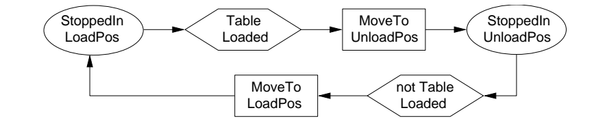
Fig. 5.4 ELEVROTTABLE ground model
