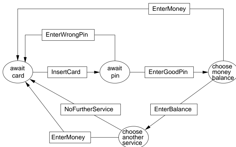
Fig. 3.1 USECASEATM model
