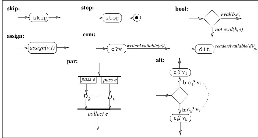
Fig. 6.20 Semantics of Occam: activity diagram ASM
