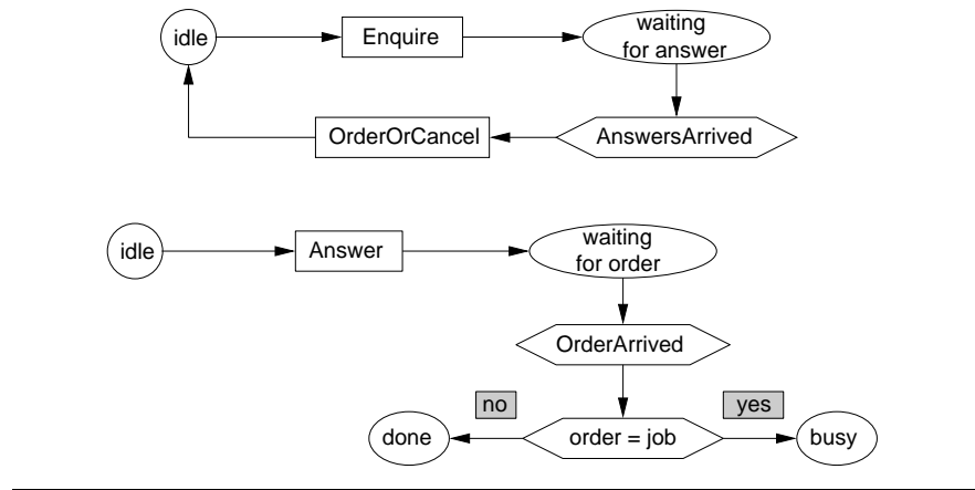
Fig. 6.3 Basic ASM of MASTER/SLAVE/AGREEMENT agents
