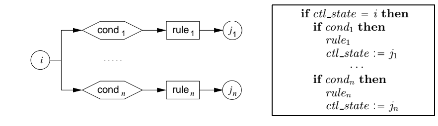
Fig. 2.6 Control state ASMs: alternative definition
