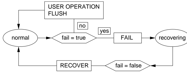
Fig. 3.12 DBRECOVERY ASM
