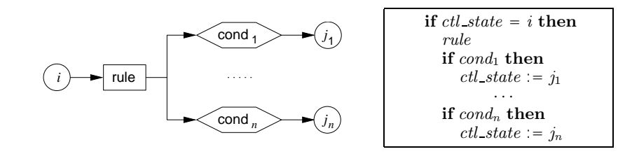
Fig. 2.6 Control state ASMs: alternative definition
