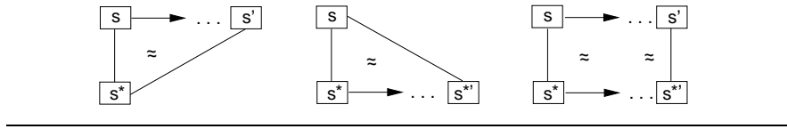
Fig. 3.13 Components of ASM refinement diagrams
