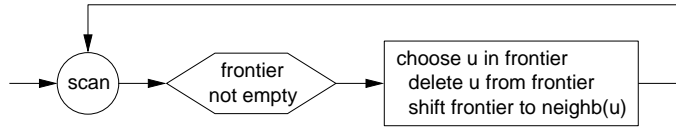
Fig. 3.9 SHORTESTPATH 2
