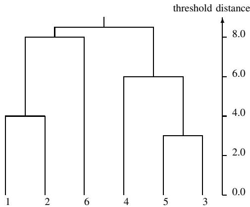
Figure 10.3 Single-link dendrogram
