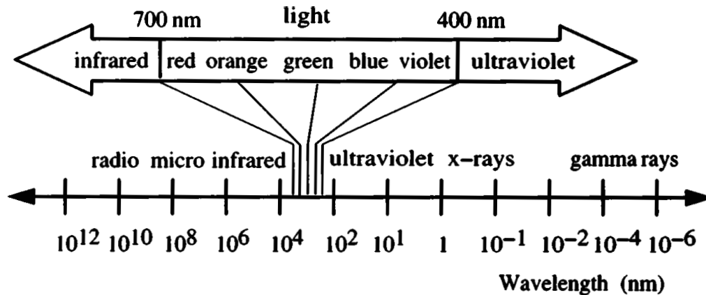
Figure 2.1: Electromagnetic spectrum.
