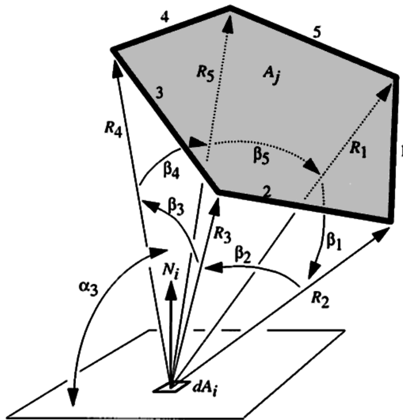
Figure 4.7: Differential area to polygon form factor.
