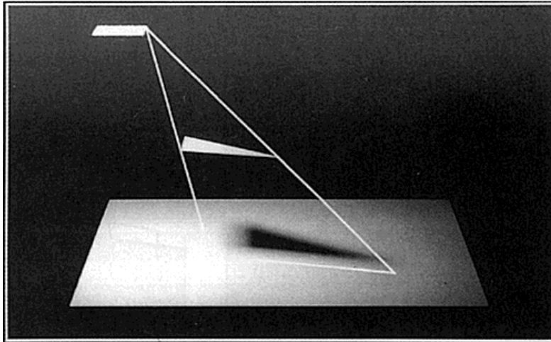
Figure 8.18: A VE event caused by a source vertex and an occluder edge. Courtesy of Daniel Lischinski and Filippo Tampieri, Program of Computer Graphics Cornell University.
