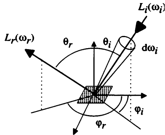
Figure 2.9: Bidirectional reflection distribution function.
