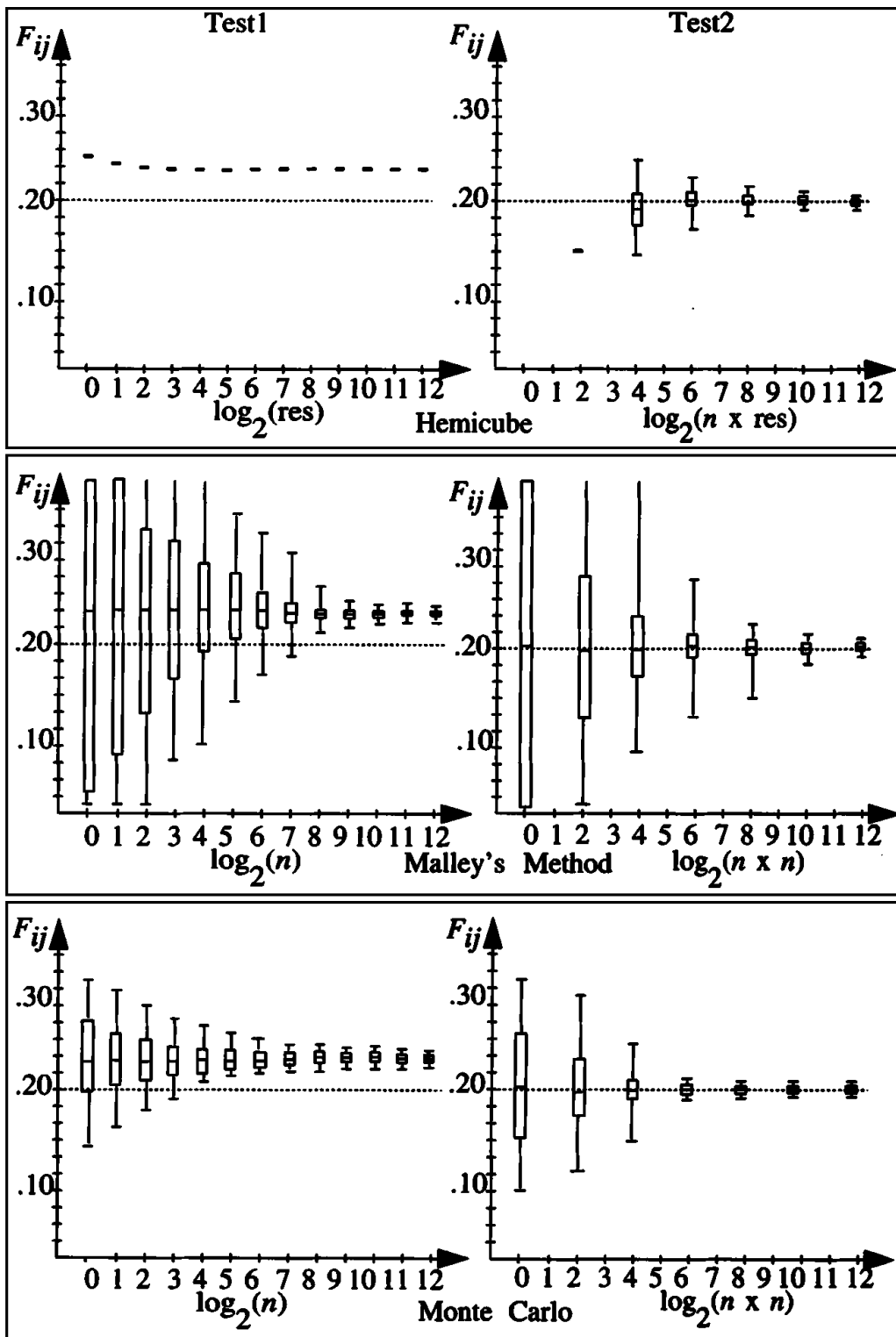
Figure 4.23: Test results on parallel elements. In Test1, only the center point was chosen on element i and n points on element j . In Test 2 n points are chosen on both elements. res is the resolution of the hemicube in both tests.
