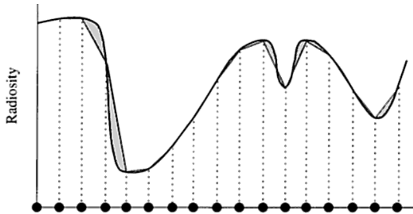
Linear elements with higher density subdivision.
