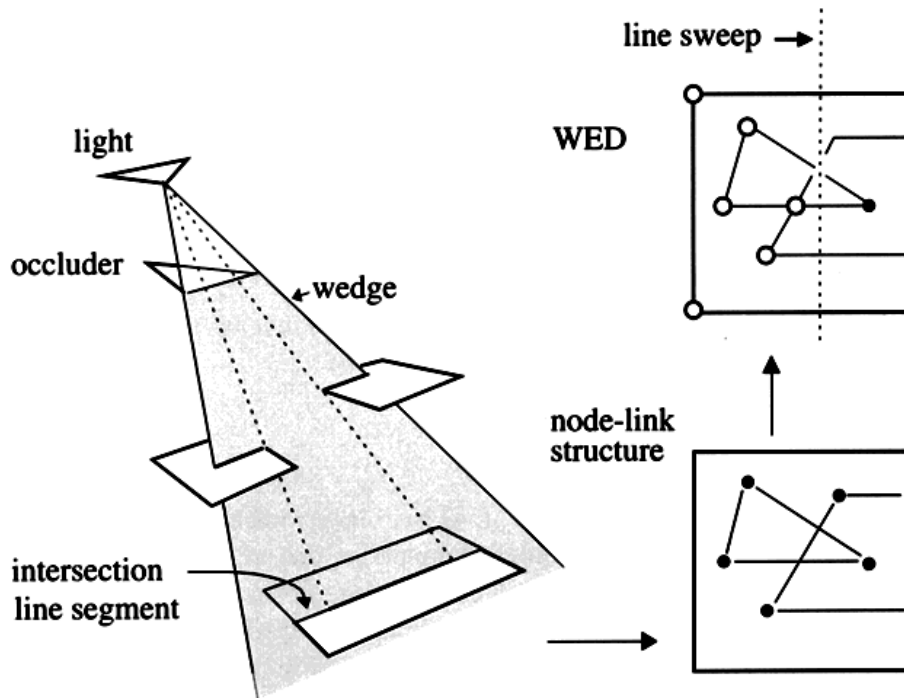
Figure 8.23: Steps in Heckbert's computation of discontinuity edges.
