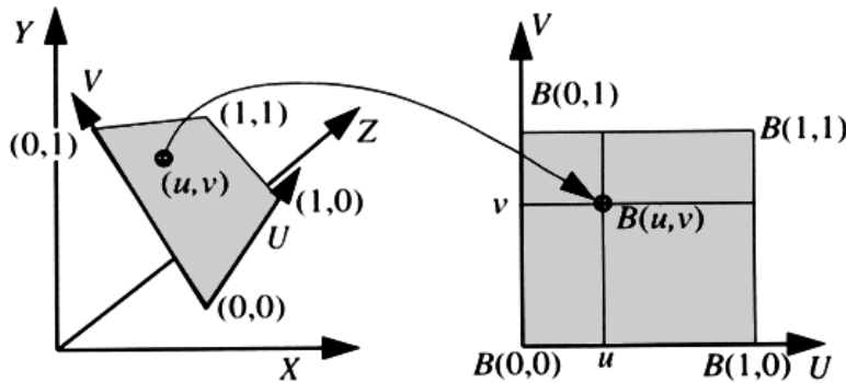
Figure 9.6: Bilinear interpolation.
