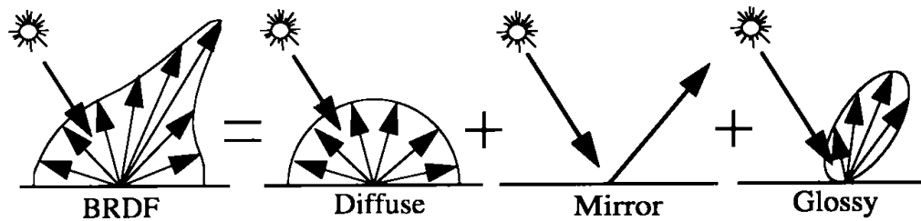
Figure 2.12: Reflectance components.
