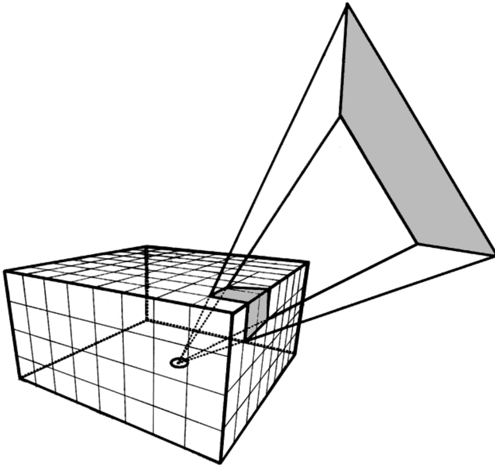
Figure 4.10: The hemicube.
