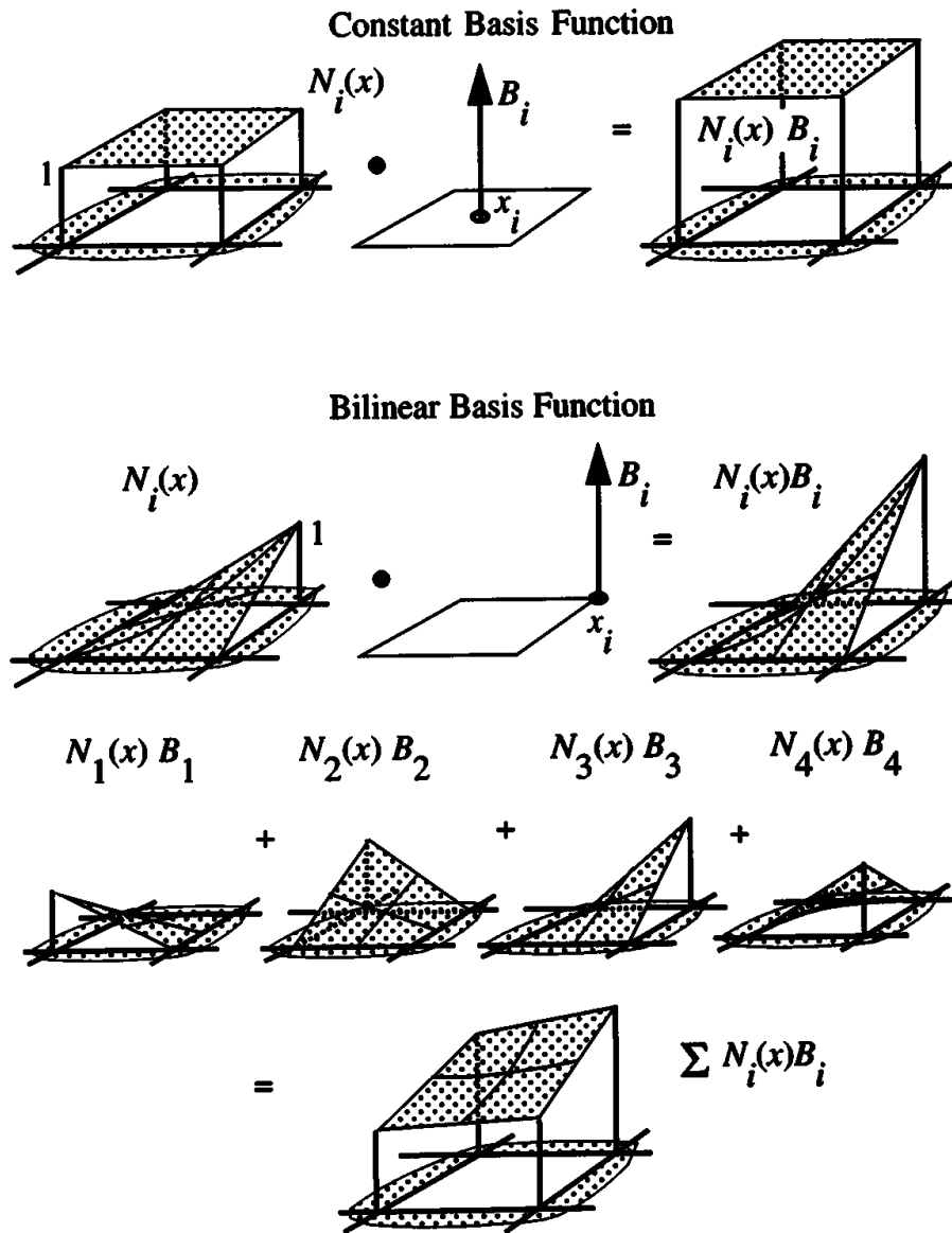
Figure 3.7: Basis functions.
