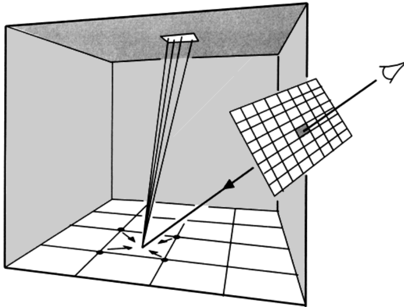
Figure 9.20: Shooting rays to compute the direct component of illumination during rendering. The direct component is interpolated from the radiosity solution.
