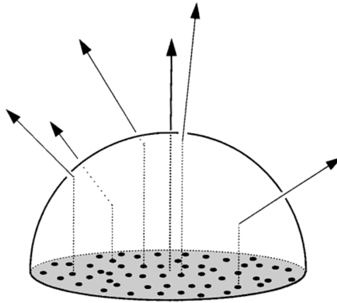
Figure 4.16: Malley's method.
